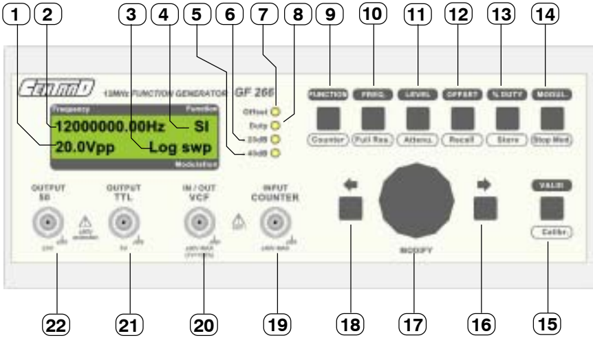
FRONTPANEL
